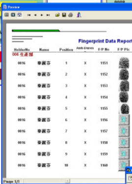
• Fingerprint Report
