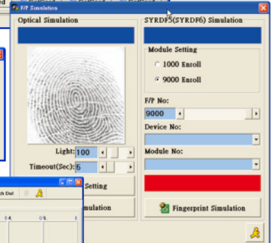
• Enroll Simulation
